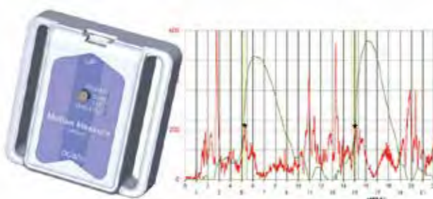
It has an acceleration sensor and an angular speed sensor built-in. The movement with a minute knee joint can be caught and digitized.
